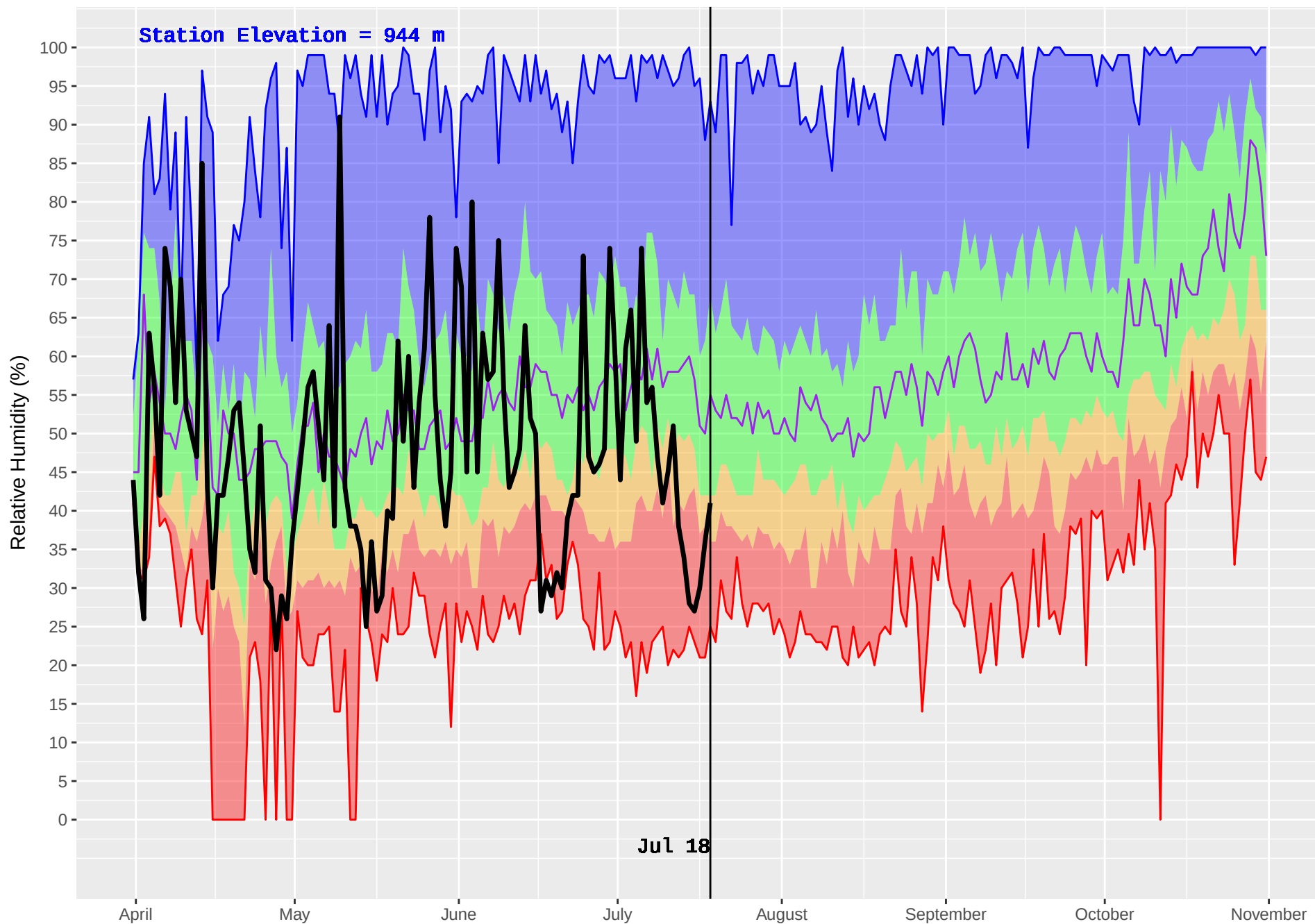
GRASSY PLAINS HUB (161) : Historical (1970–2016) and Current (2018) Daily Relative Humidity
